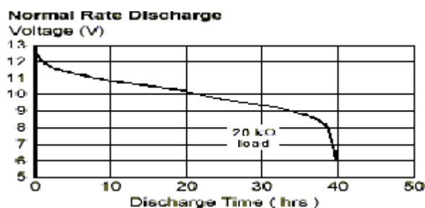
Typical Discharge characteristics at 22 ± 3 °C
