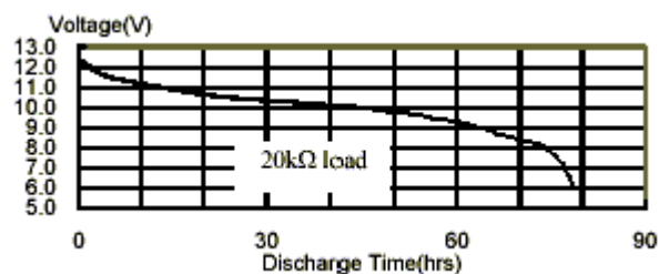
Typical Discharge characteristics at 22 ± 3 °C
